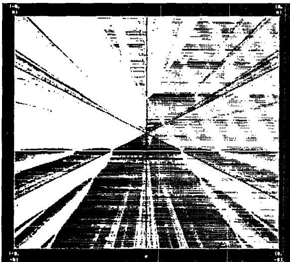
FIG. 3. This is the basin map associated with M_{0.5} . The three invariant lines form a triangle and the singular lines cross through the origin.
