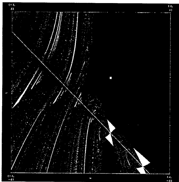
FIG. 1. This is a basin map for the bow tie phenomena in the B_{0.75} map. The white points have been mapped to the bow tie within 200 iterations.
